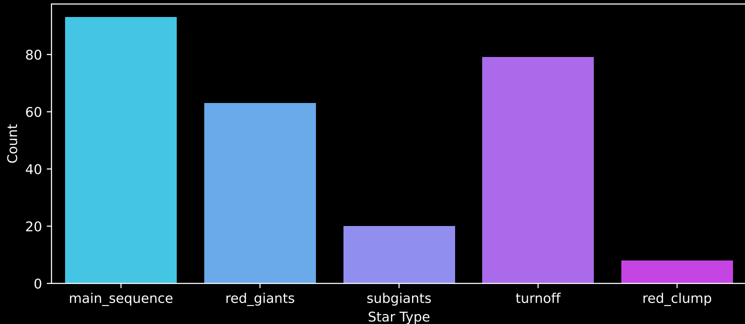
GALAH DR4 Field: [2848] Count plot of Star Type
