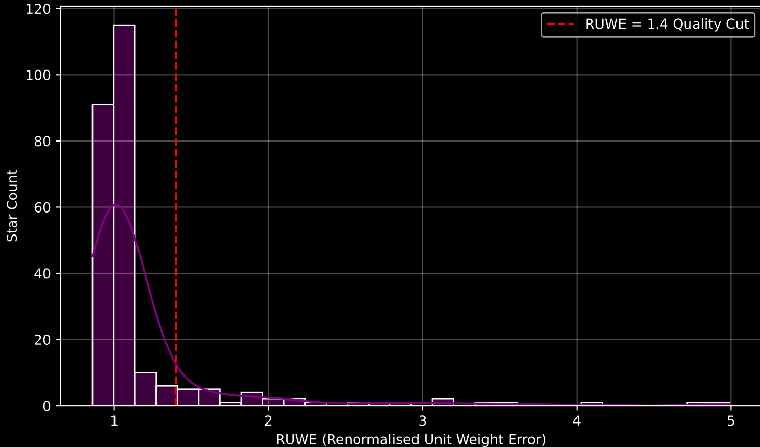
GALAH DR4 Field [2848] RUWE Distribution (n= 252)
