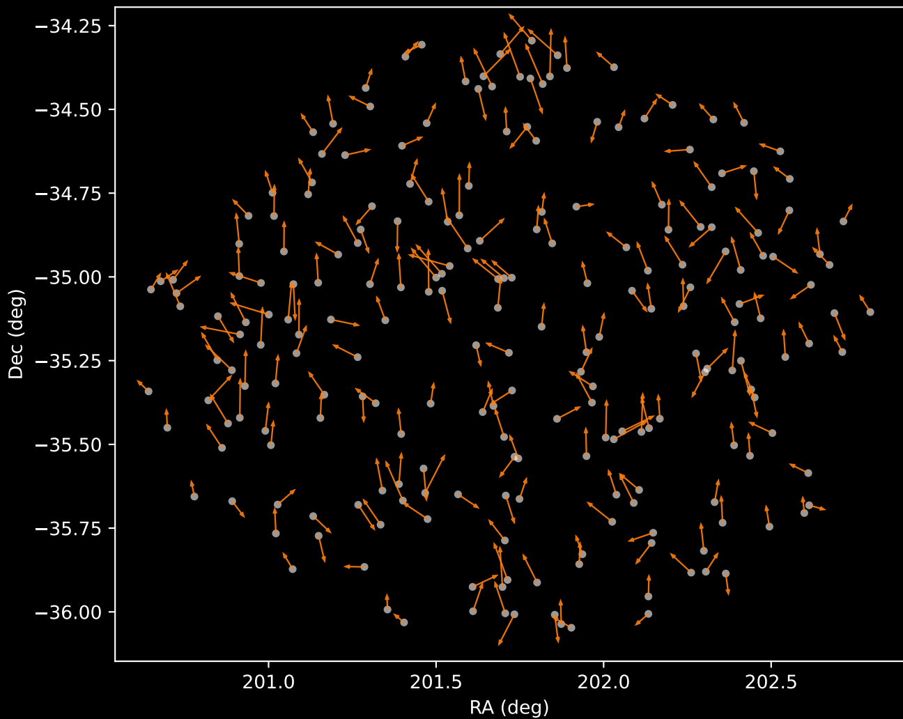
GALAH DR4 Cluster 2 Proper Motion Vectors (n=224)
