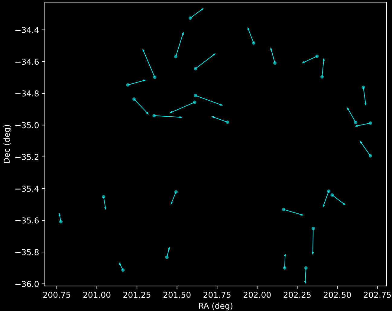
GALAH DR4 Noise Stream Proper Motion Vectors (n=29)
